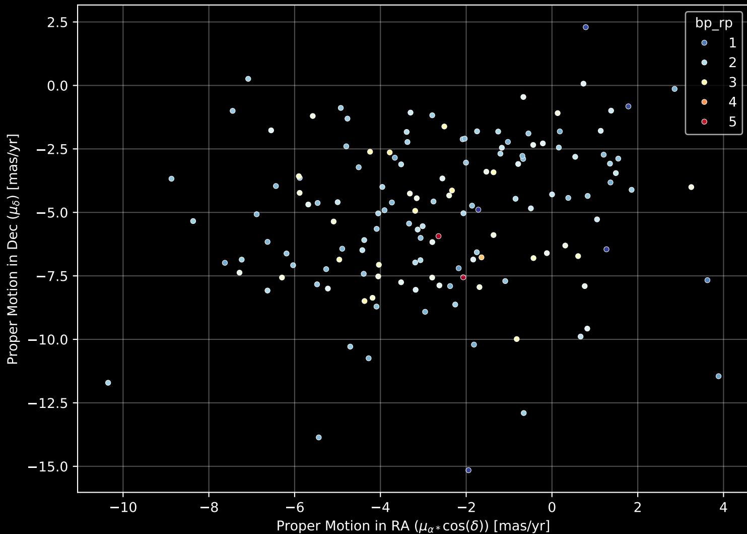
APOGEE DR17 Field: [005+05-O] Proper Motion Diagram (n= 145)
