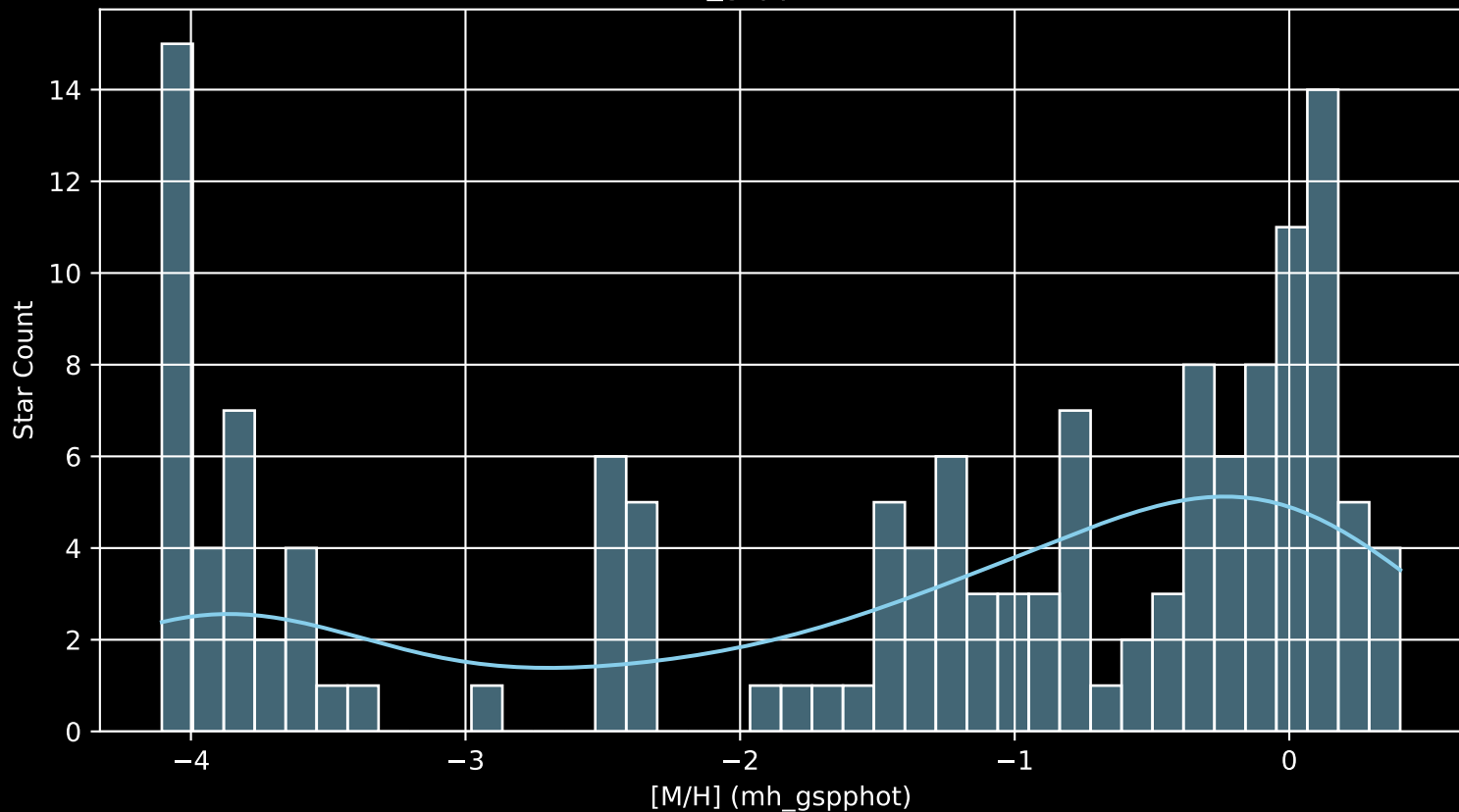
APOGEE DR17 Field: [005+05-O [M/H] (mh_gspphot) (n= 143)
