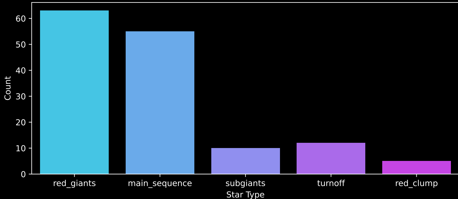
APOGEE DR17 Field: [005+05-O] Count plot of Star Type
