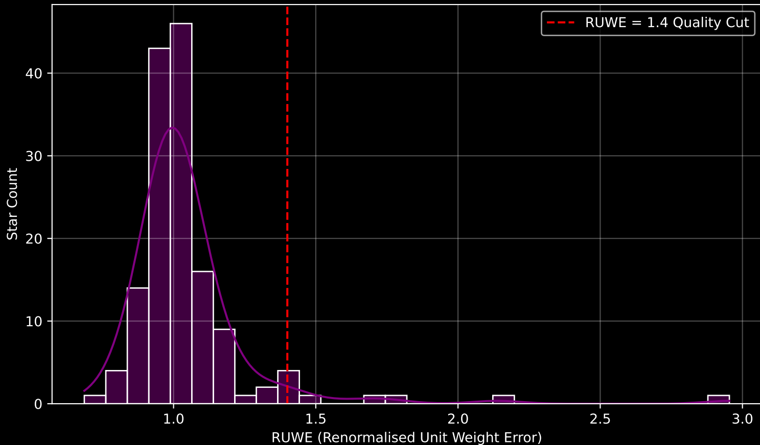
GAPOGEE DR17 Field [005+05-O] RUWE Distribution (n= 145)
