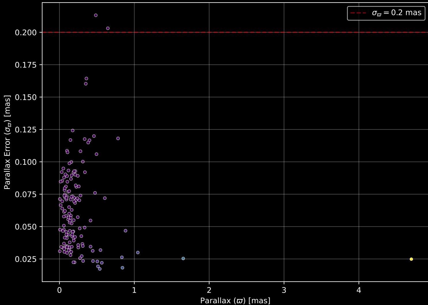
APOGEE DR17 Field: [005+05-O] Parallax Quality (n= 145)
